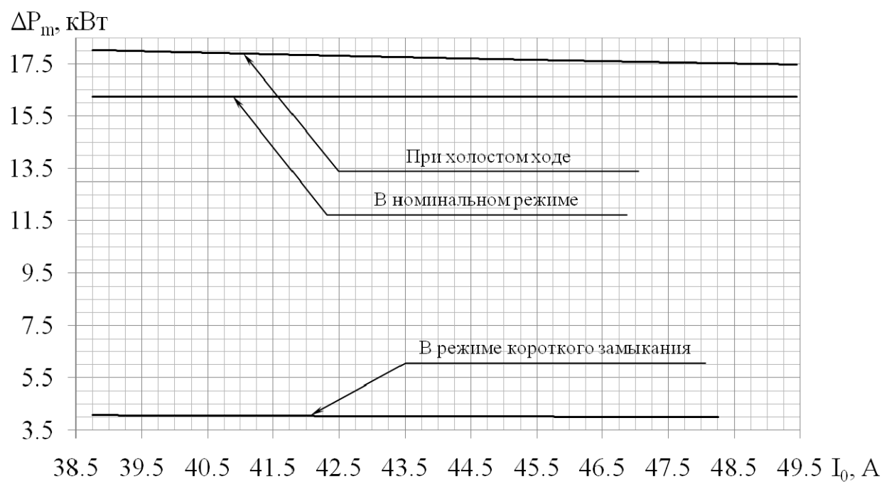
Fig. 8. Dependence of magnetic losses on the magnetizing current
