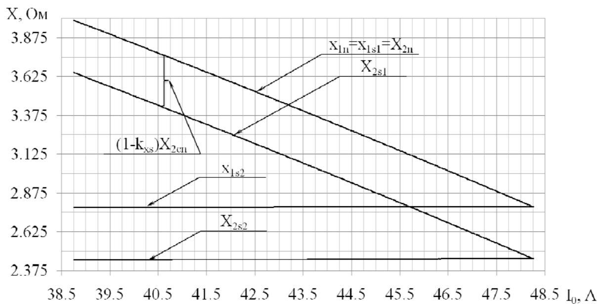
Fig. 6. Dependence of dispersion inductive resistances on the magnetizing current
