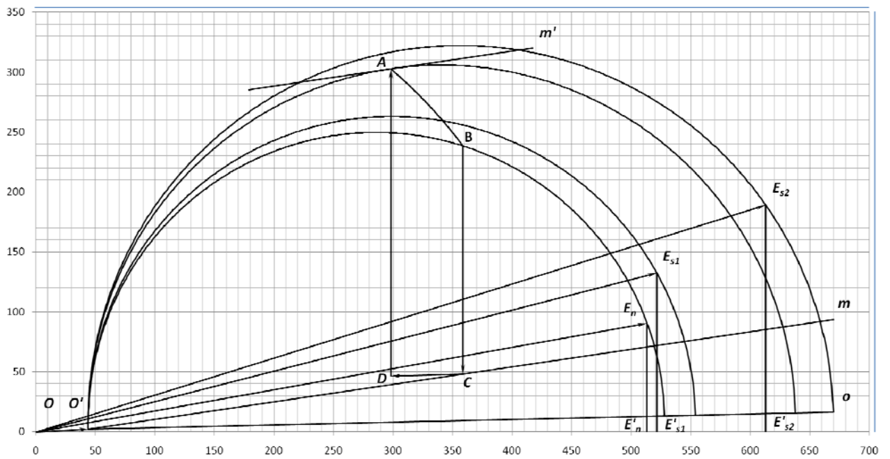
Fig. 3. Circular graph for determination of critical moment
