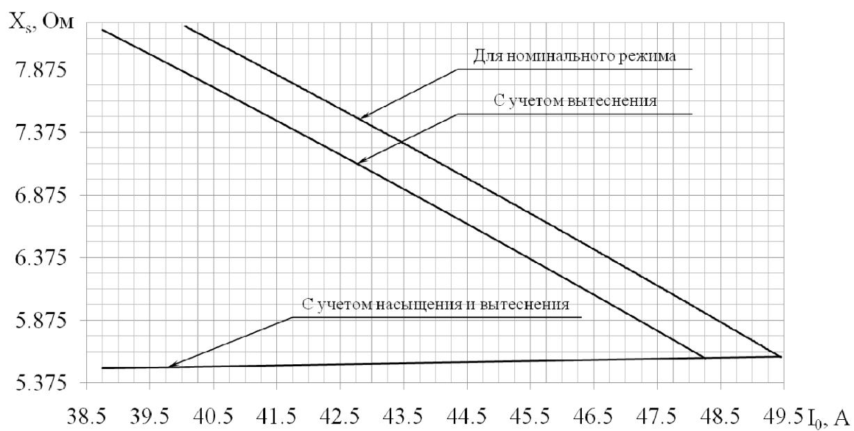
Fig. 5. Dependence of short circuit inductive resistance on the magnetizing current
