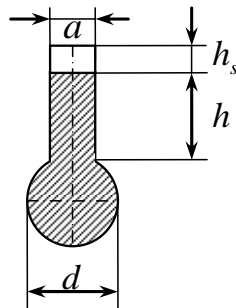
Fig. 2. Cross-sectional sketch of retort slot
