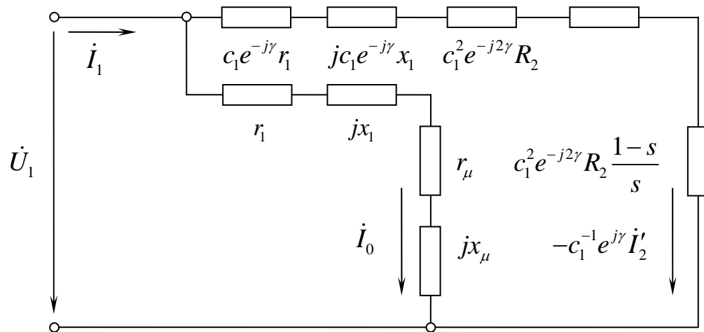
Fig. 1. L-type chart of substituting for an asynchronous machine
