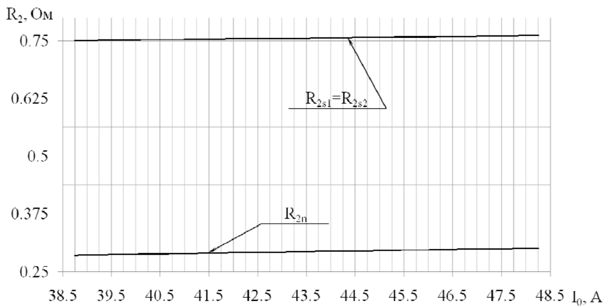
Fig. 7. Dependence the brought pure resistance over of rotor on the magnetizing current
