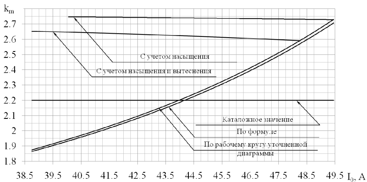
Fig. 4. Dependence of critical torque multiplicity on the magnetizing current
