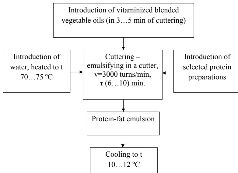
Fig. 1. Technological scheme of preparing PFE
